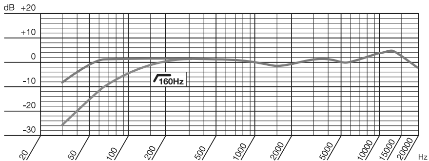
Frequenzgang C214
