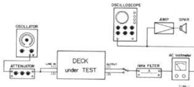
Fig. 8-13 Test Connections for Erase Measurement
