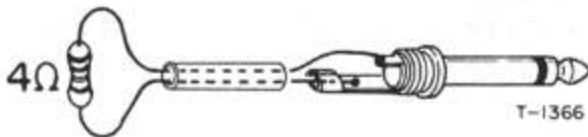
Fig. 8-7 Test Connections for Headphone Output Check
