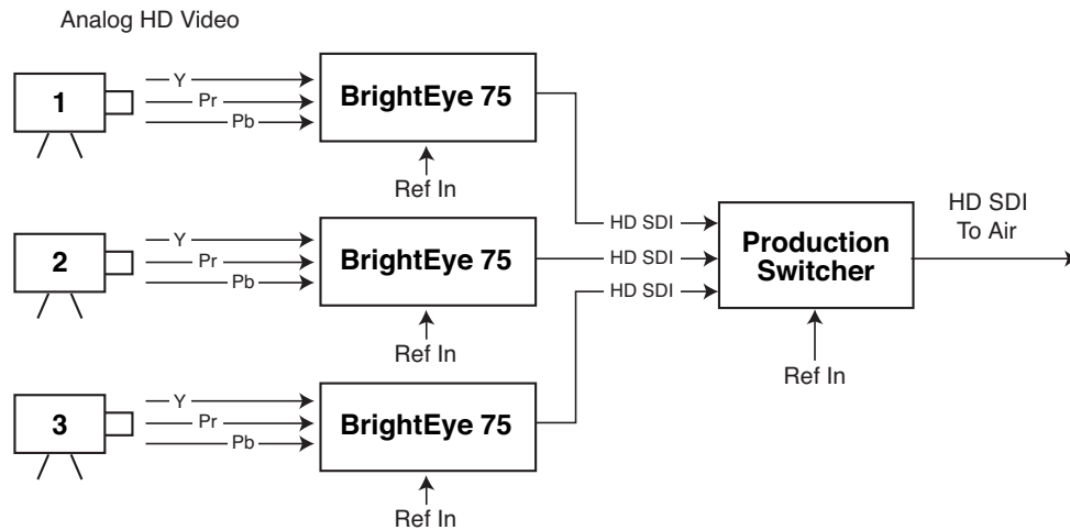
BrightEye 75 Signal Ingest Application for HD Signals
