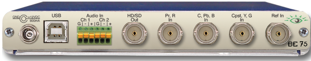
BrightEye 75 Rear Connectors
