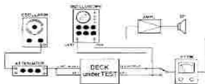
Test Connection for Recording Check
