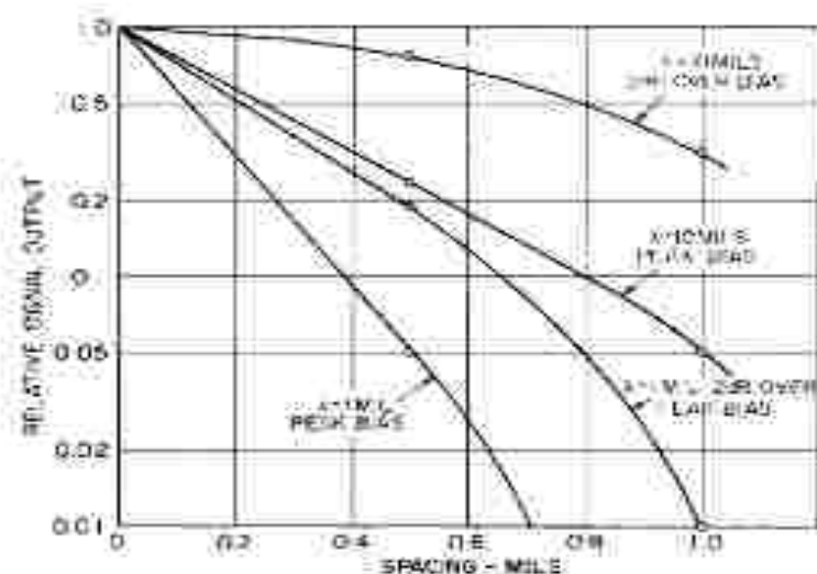
Fig. 2-8 Curves showing the fall off of recorded signals versus spacing from recording head. (Courtesy, Minnesota Mining and Manufacturing Co.)
