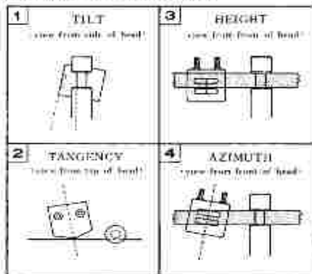
Fig. 2-21 Head Mis-Alignment Example
