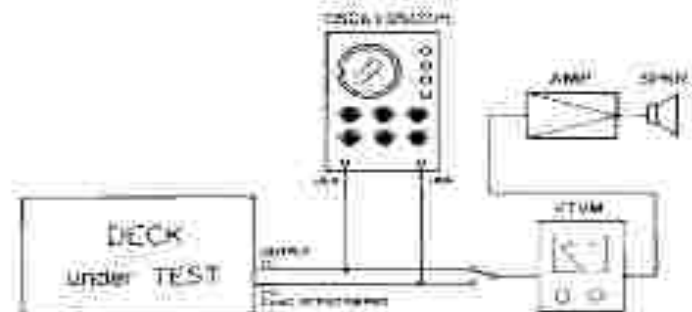
Fig. 2-20 Head Alignment Fine Adjustment Set-up and Test Connections (REPRODUCE)
