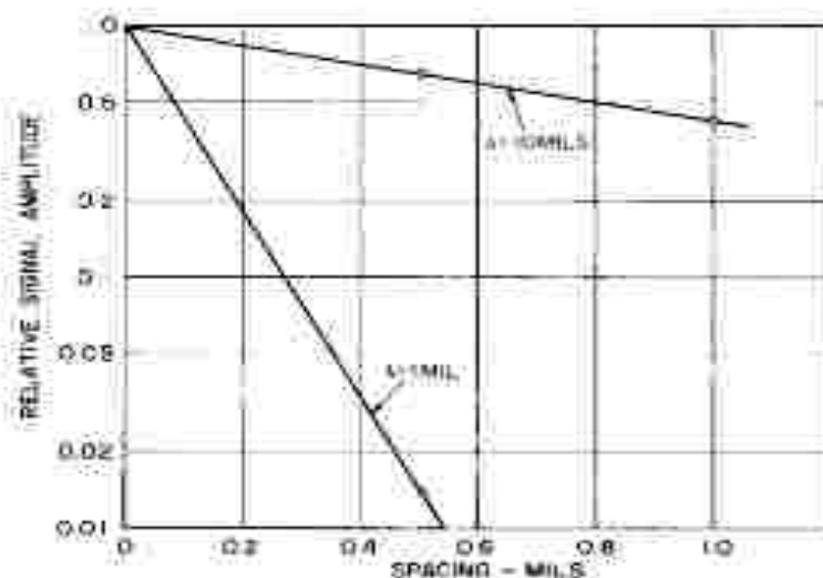
Fig. 2-7 Curves showing fall-off of reproduced signals versus spacing from reproducer head. (Courtesy, Minnesota Mining and Manufacturing Co.)
