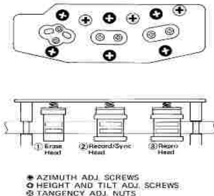
Fig. 2-25 Head Adjustment Screws and Alignment
